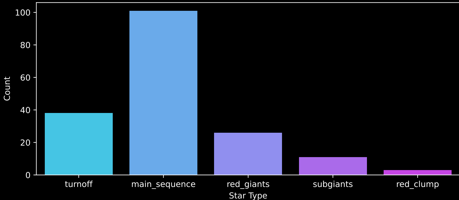
APOGEE DR17 Field: [053+88_MGA] Count plot of Star Type
