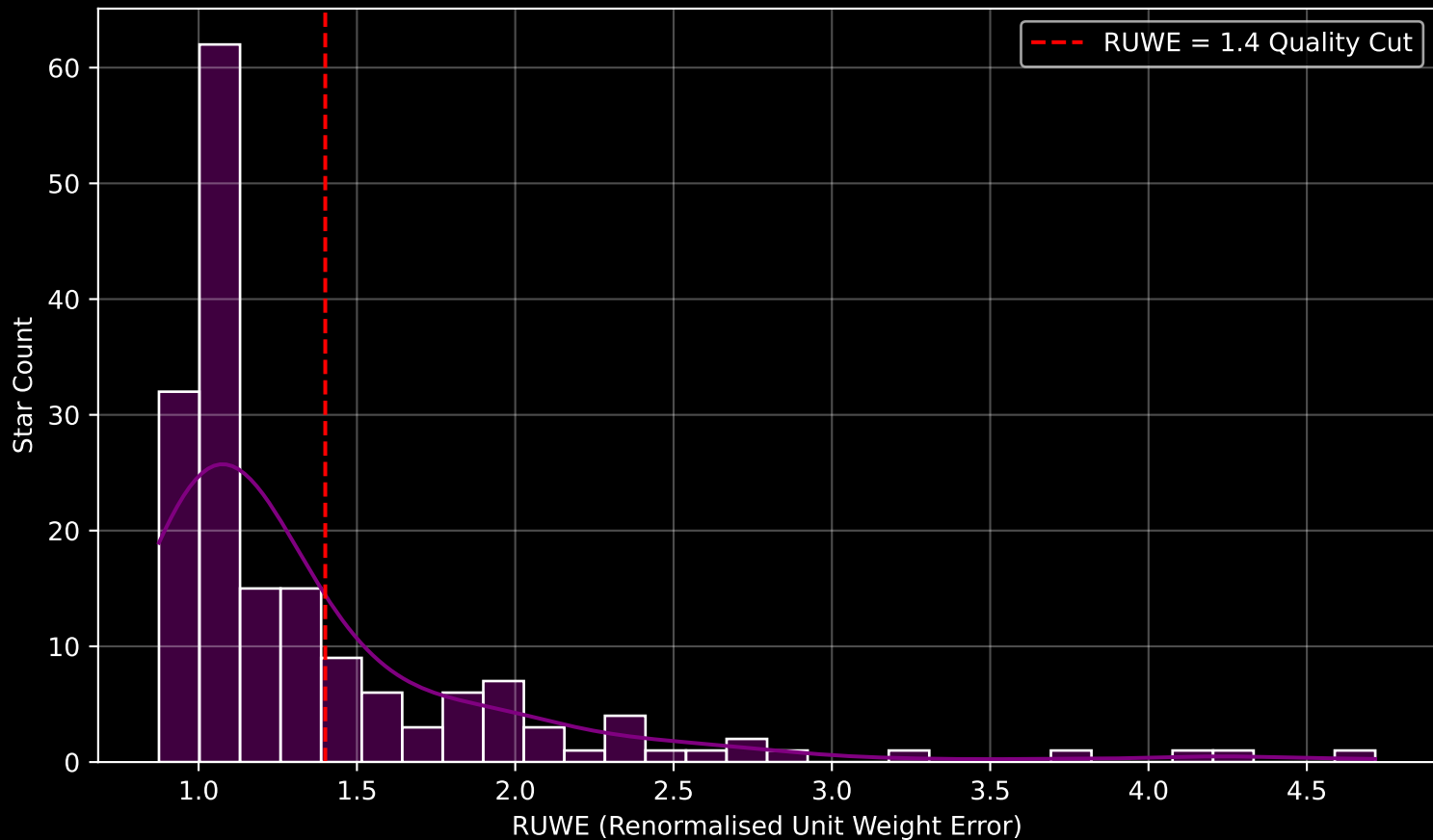
GAPOGEE DR17 Field [053+88_MGA] RUWE Distribution (n= 173)
