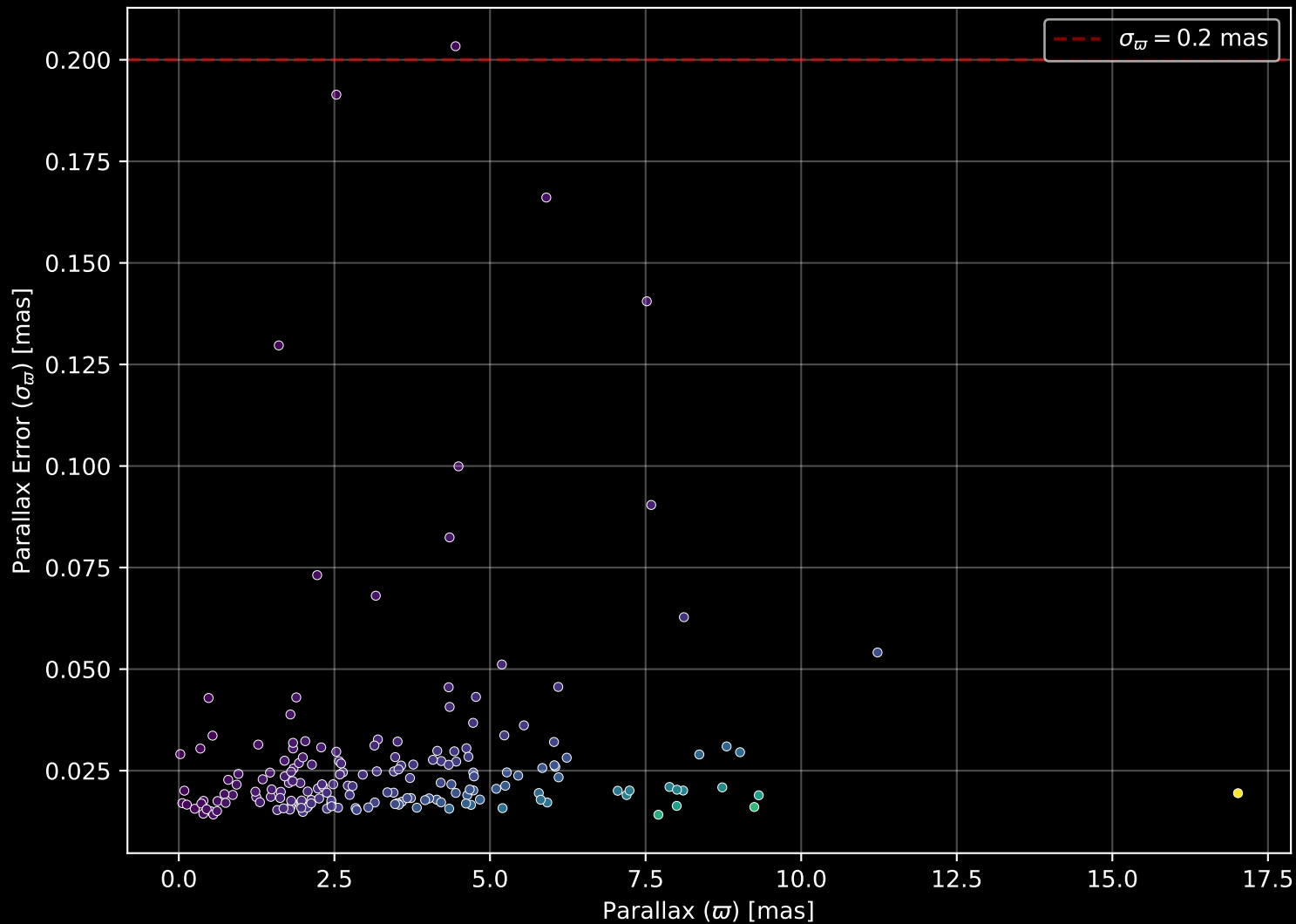
APOGEE DR17 Field: [053+88_MGA] Parallax Quality (n= 179)
