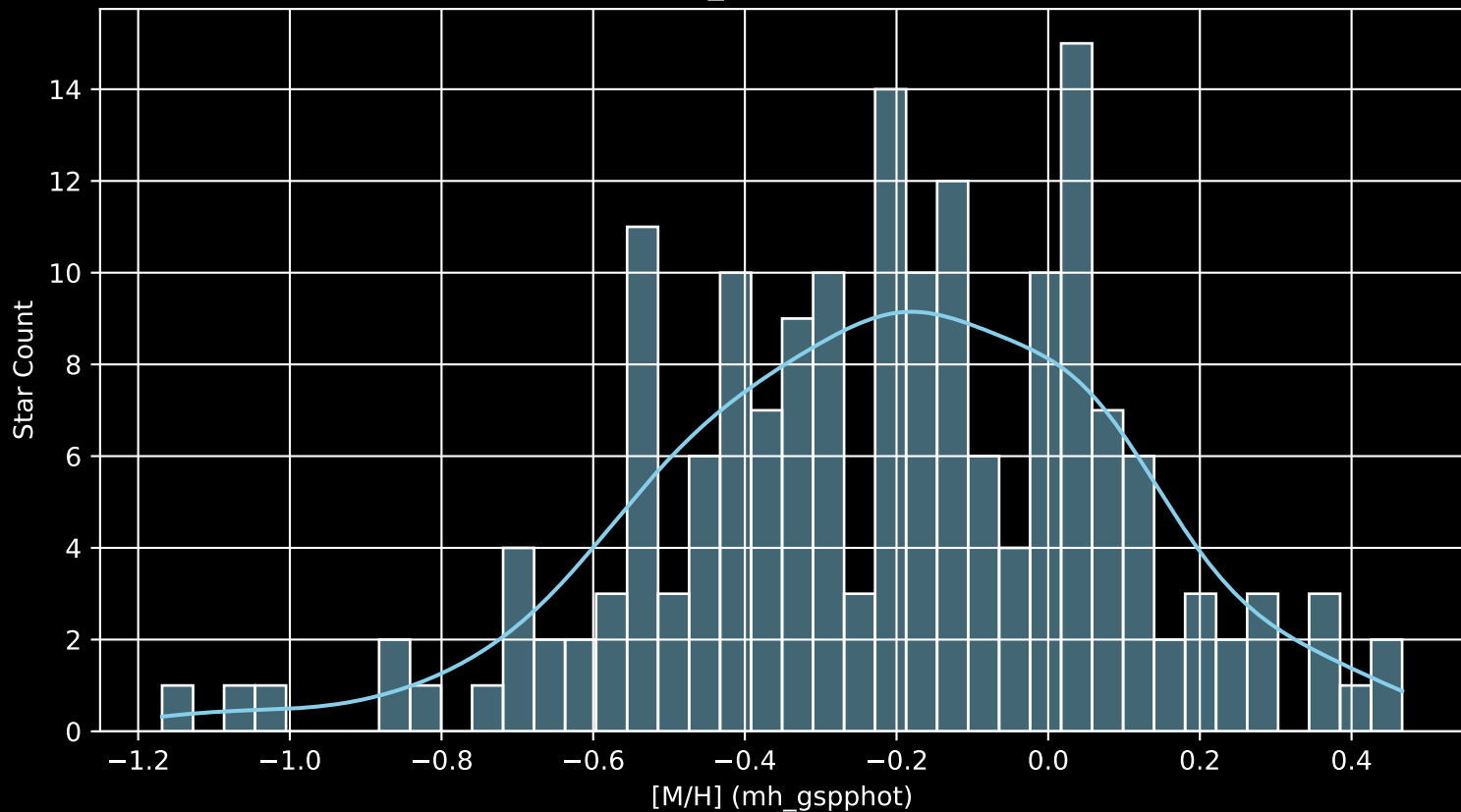
APOGEE DR17 Field: [053+88_MGA [M/H] (mh_gspphot) (n= 177)
