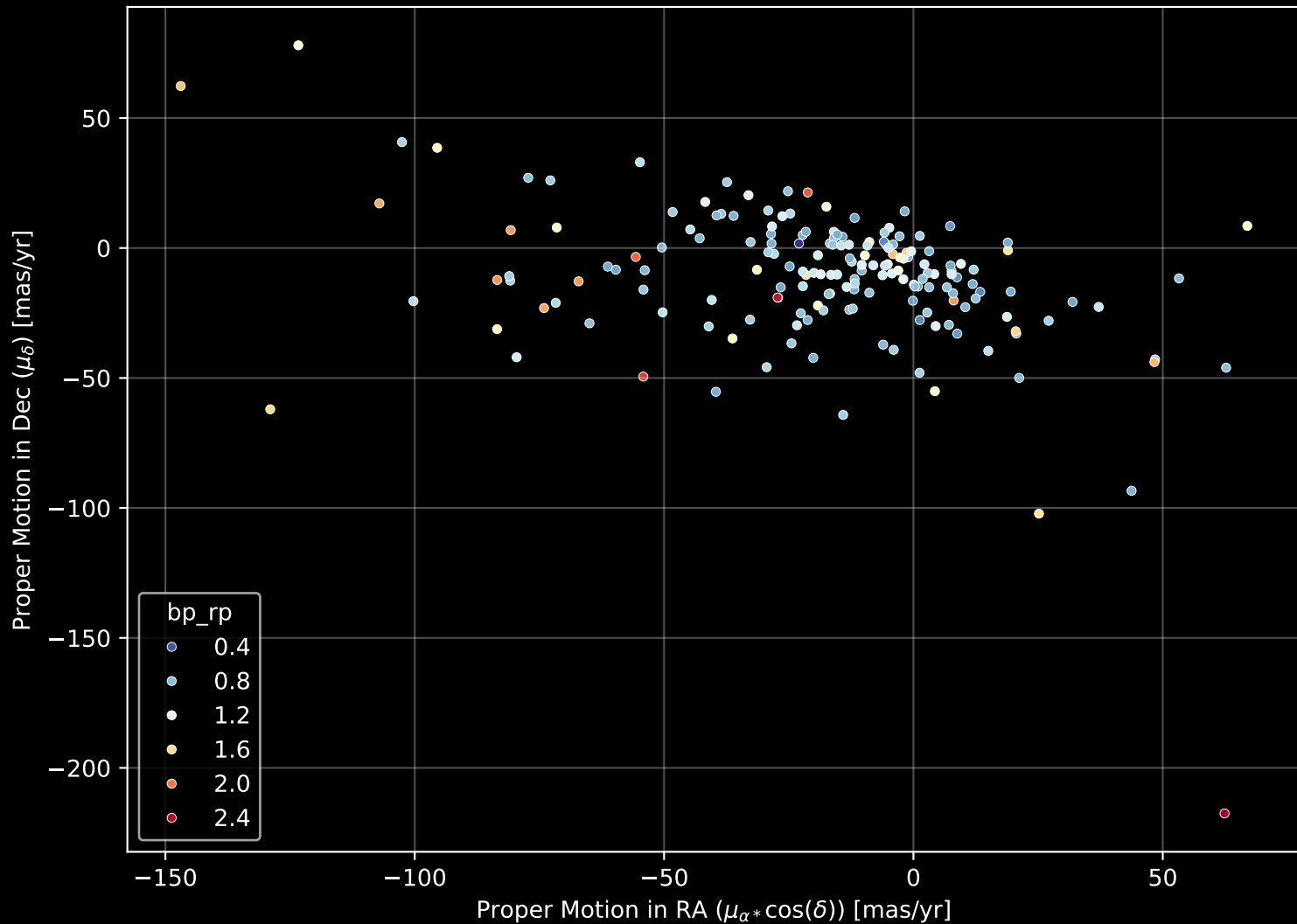
APOGEE DR17 Field: [053+88_MGA] Proper Motion Diagram (n= 179)
