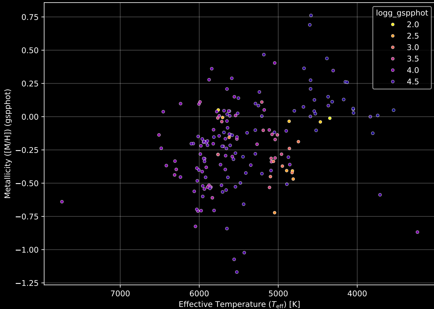
APOGEE DR17 Field: [053+88_MGA] Stellar Population Parameters (n= 179)
